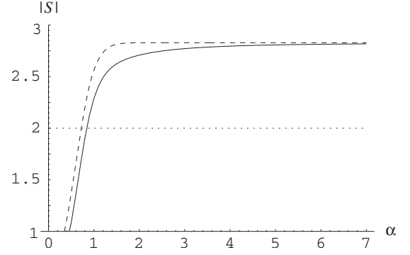
FIG. 5. The numerically optimized Bell parameter |S| for an ECS with amplitude \alpha using the real local operation (solid curve) and the ideal local operation (dashed curve). See text for details.
